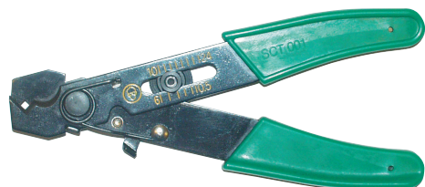
Stripping tool SCT001, cuts and strips 0.5-6 mm 2
